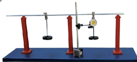
PIN JOINT TRUSS APPARATUS
