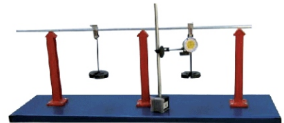
DEFLECTION OF BEAM APPARATUS
