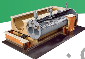
LANCHISHER BOILER
