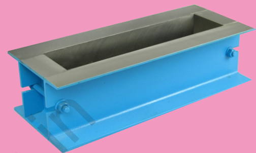
BEAM MOULD
