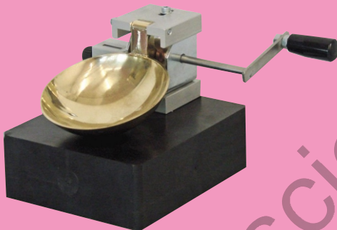
LIQUID LIMIT APPARATUS
